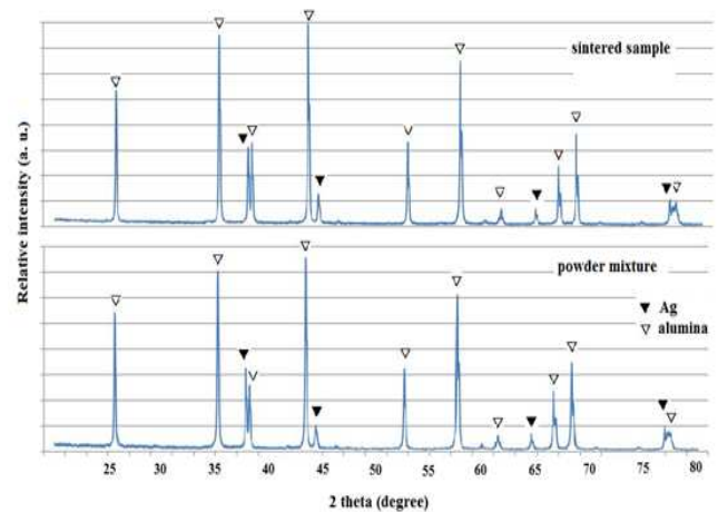
Figure 2. X-ray diffraction patterns of powders mixture after milling and sintered sample at 1500°C, during 1h.
